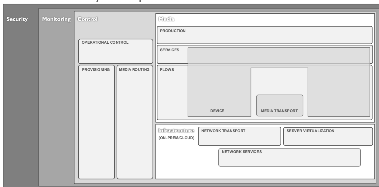
Illustration 1 Networked Media Systems Template – Overview
