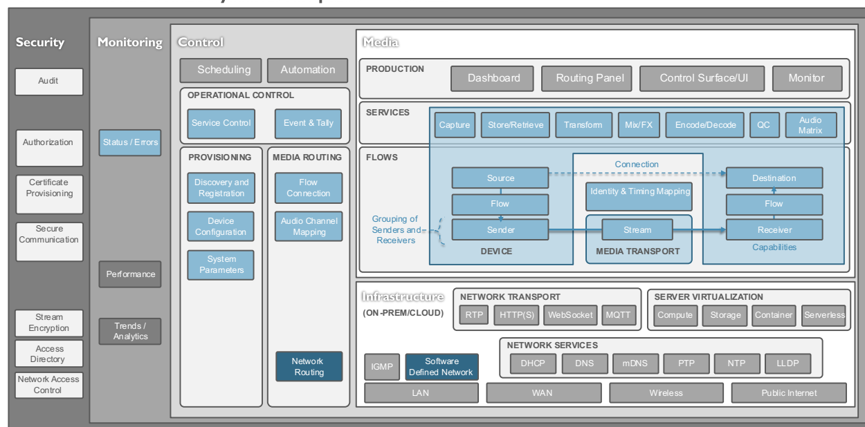
The Networked Media Systems Template — Detail
