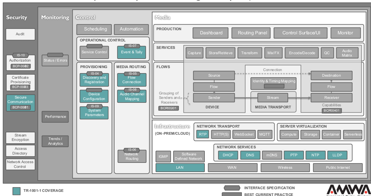
Illustration 4 Networked Media Systems Template – Showing the Scope of JT-NM TR-1001-1
